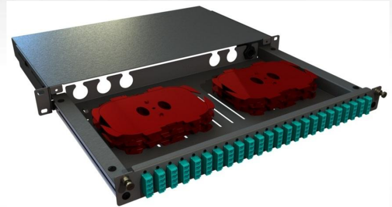
Standard LC Quad Plate with New Splice Cassettes with integrated fibre management.
